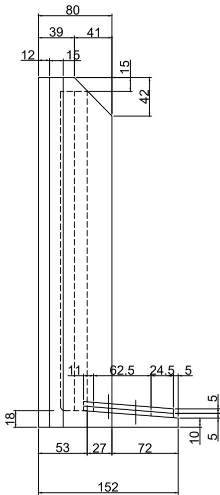
VIEW "A"
