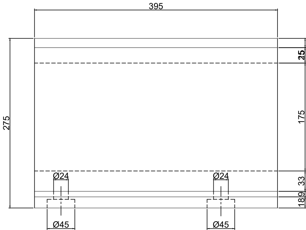
VIEW "B"
