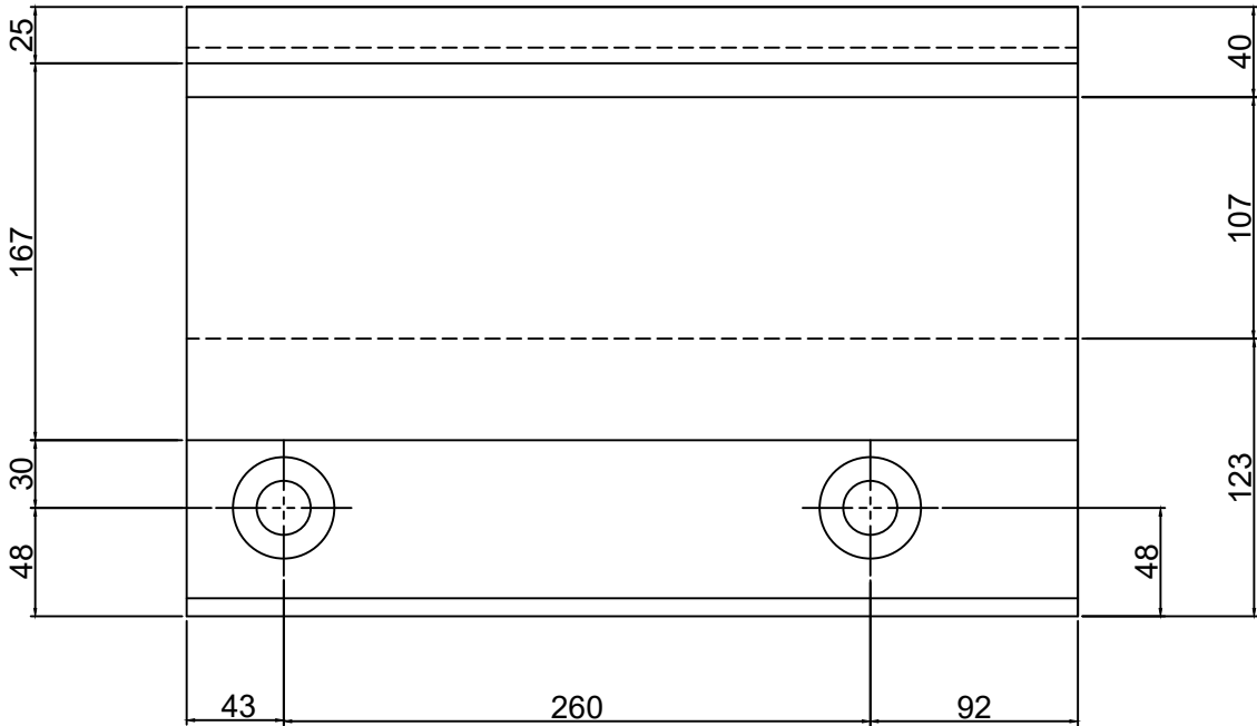
VIEW "A"
