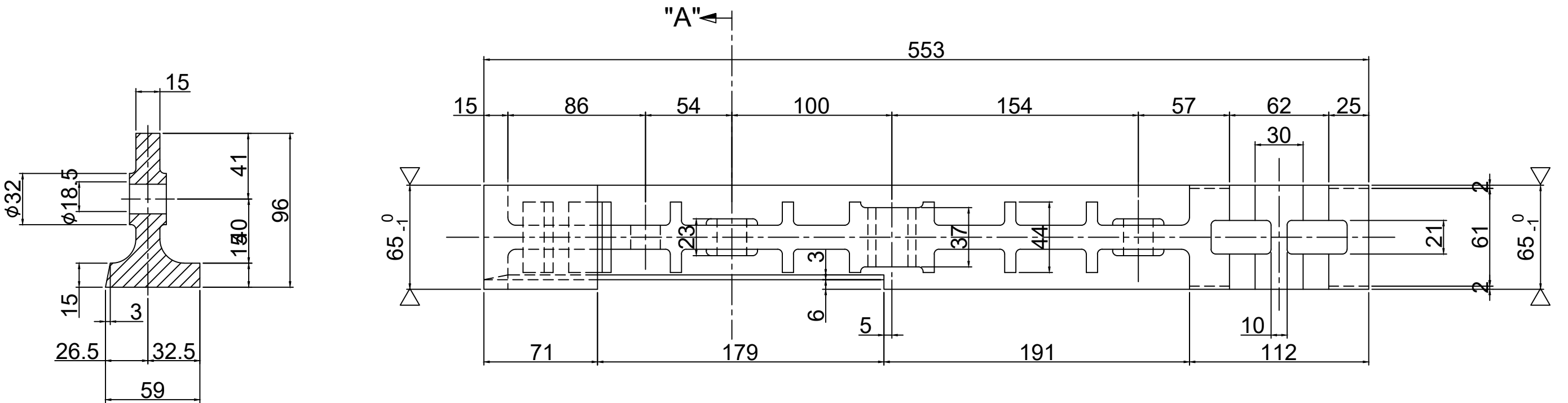
SECTION "A"
