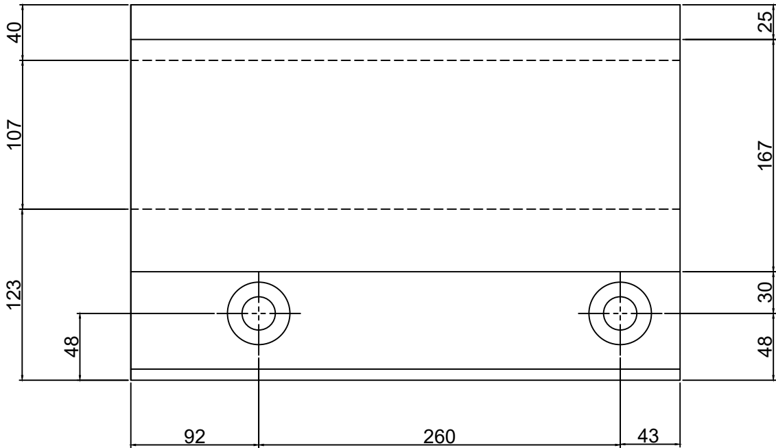
VIEW "A"
