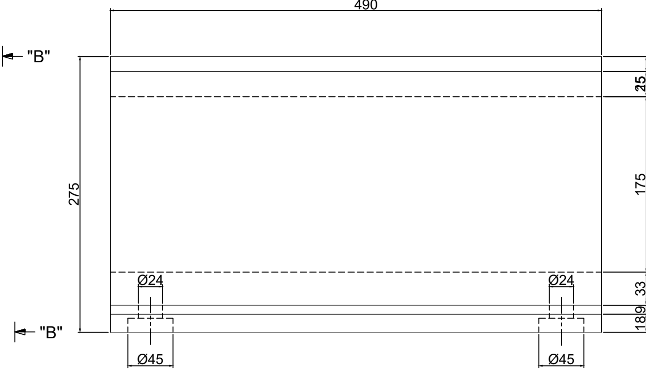
VIEW "B"
