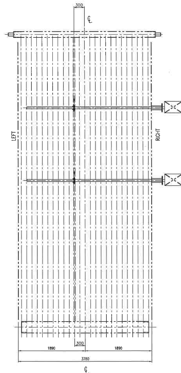
EVAPORATOR FRONT VIEW
