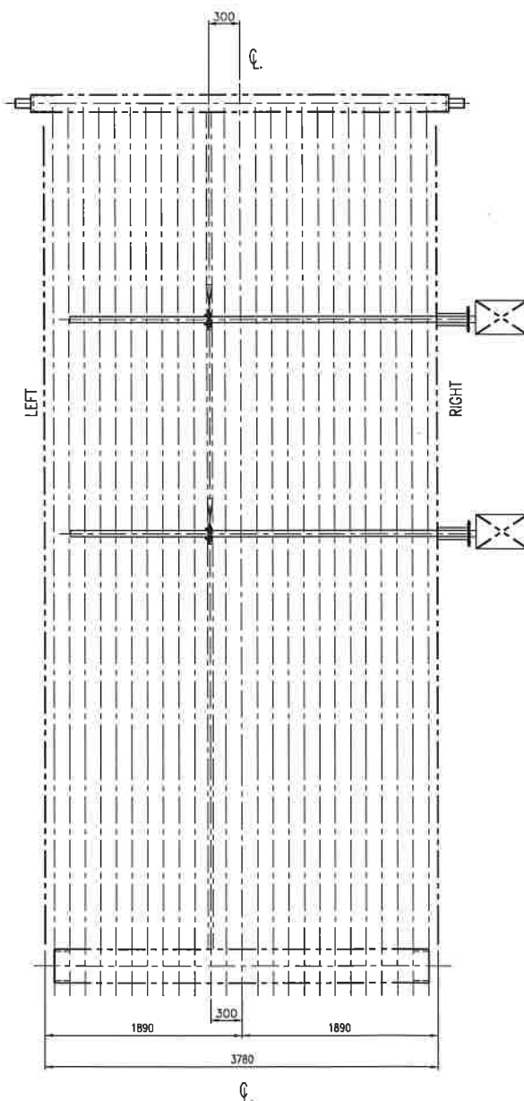
EVAPORATOR FRONT VIEW
