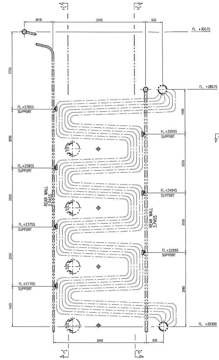
EVAPORATOR SIDE VIEW (RIGHT VIEW)
